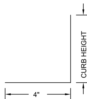
ANGLE FLASHING
