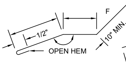
TRANSITION FLASHING
