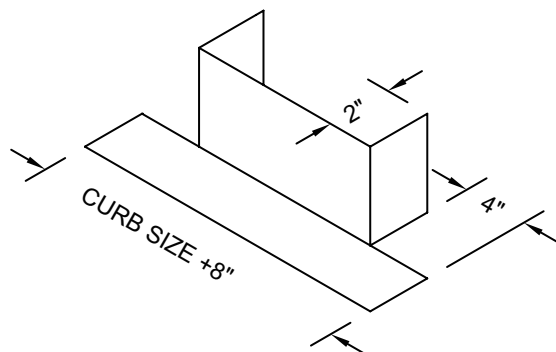
WRAP FLASHING
