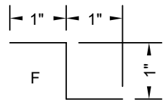
ZEE CLOSURE
