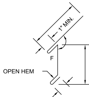
DRIP FLASHING
